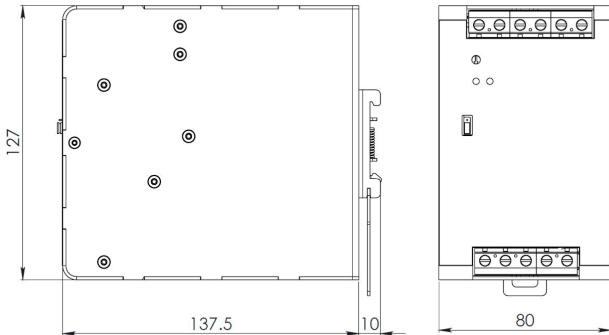
Figure 1. Mechanical Drawing
