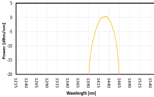
FIG. 5: SLED 4 SPECTRUM
