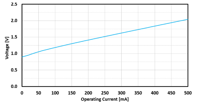
FIG. 16: SLED 5 FORWARD VOLTAGE VS CURRENT
