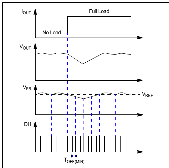
FIGURE 4-2: MIC28516 Load Transient Response.
