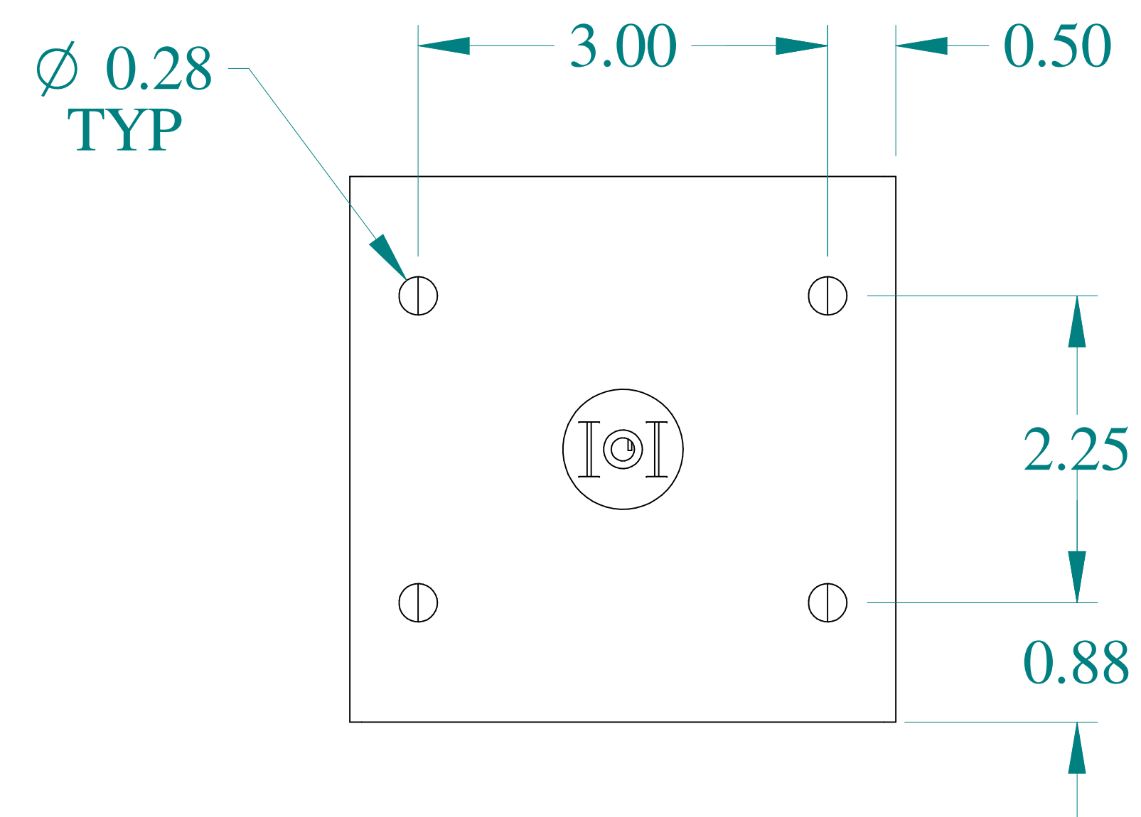
BOTTOM VIEW
