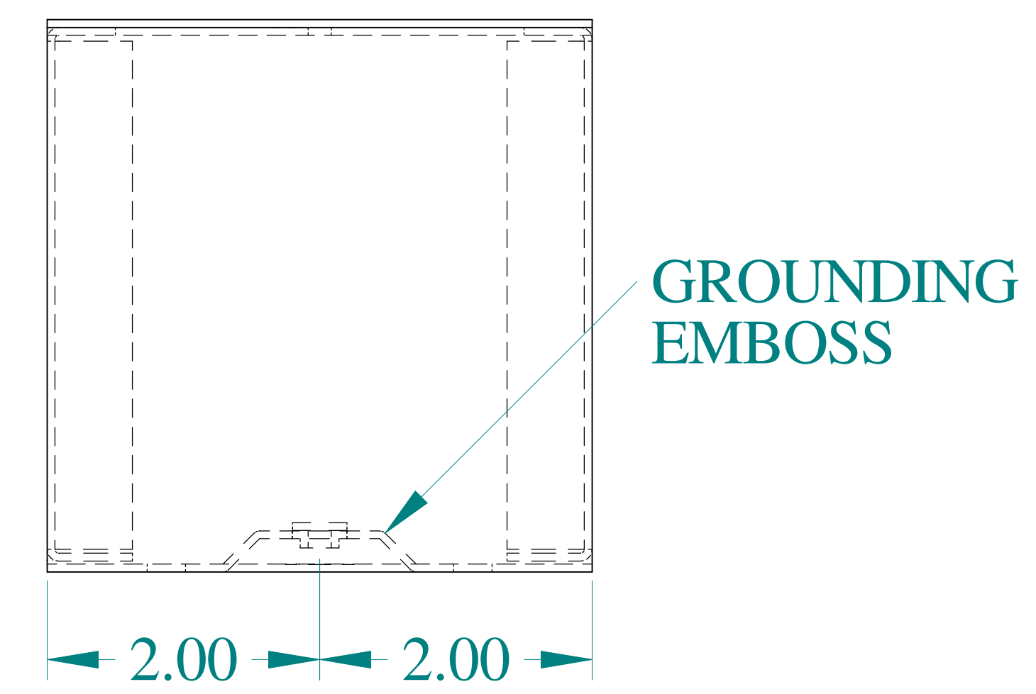
SIDE VIEW
