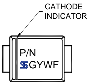
DETAIL A, ROTATED -90° (SCALE 2:1)
