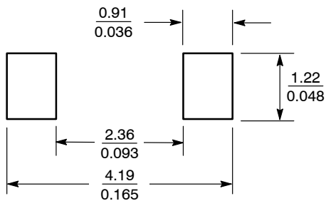
SCALE 10:1 (mm/inches)
