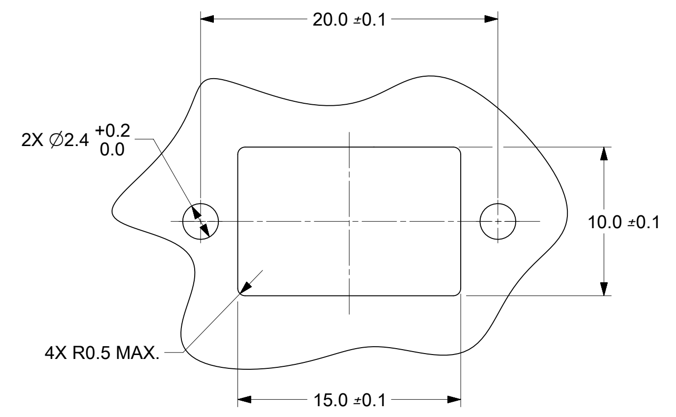
RECOMMENDED MOUNTING PATTERN
