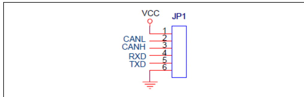
FIGURE 2-2: PINOUT FOR THE SCREW-IN TERMINALS
