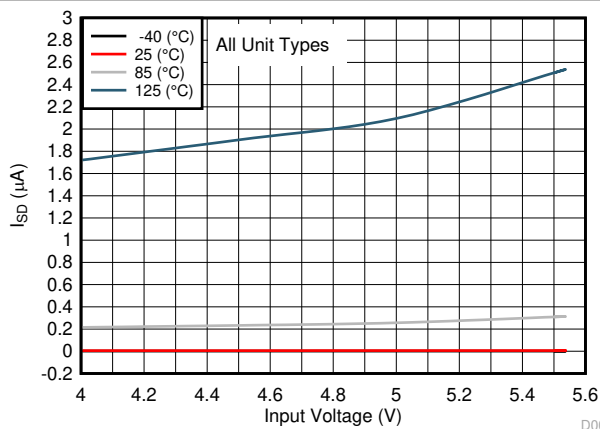
Figure 6-11. Disabled Supply Current (I sd ) vs Input Voltage
