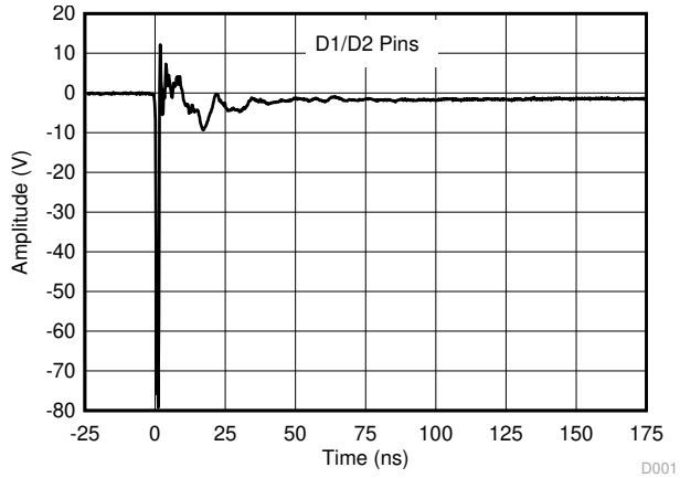
Figure 6-19. D1/D2 IEC 61000-4-2 –8-kV Contact D001
