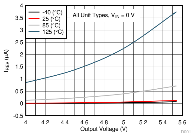
Figure 6-12. Reverse Leakage Current (I rev ) vs Output Voltage
