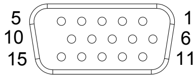
Figure 2.18 VGA Connector
