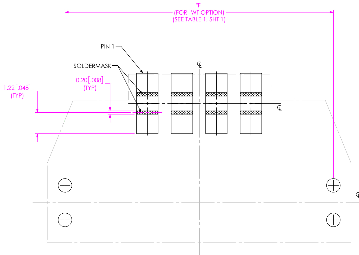
FIG 5 UMPT-04-01-XXX-RA-WT-M FOOTPRINT SHOWN (DIFFERENT AS SHOWN, OTHERWISE SAME AS FIG 1) (NOT RELEASED)
