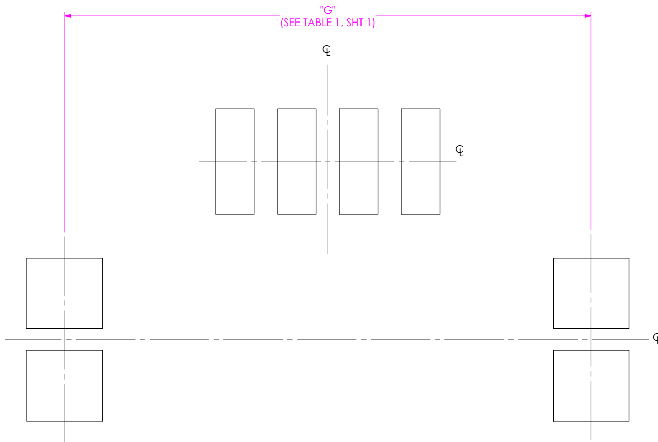
FIG 6 UMPT-04-01-XXX-RA-WT-M STENCIL SHOWN (DIFFERENT AS SHOWN, OTHERWISE SAME AS FIG 1 & 2) (NOT RELEASED)
