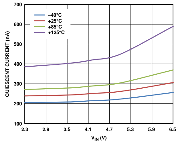
Figure 15. Hysteresis Quiescent Current vs. V_{IN\ SYNC/MODE} = \text{Low}
