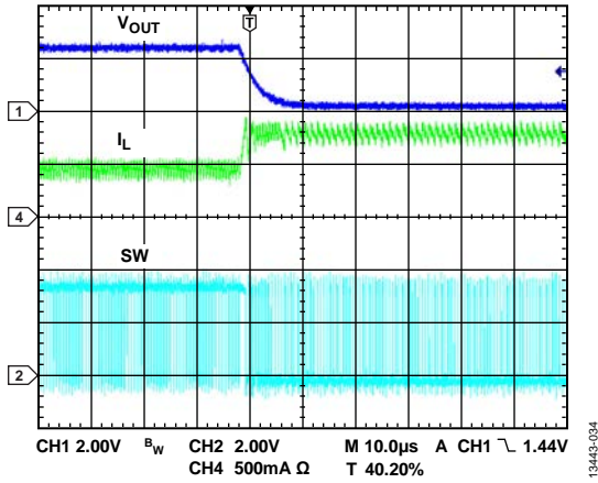
Figure 34. Output Short
