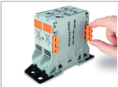
Optionally, insert block-to-block connector (285-168) into housing slot.
