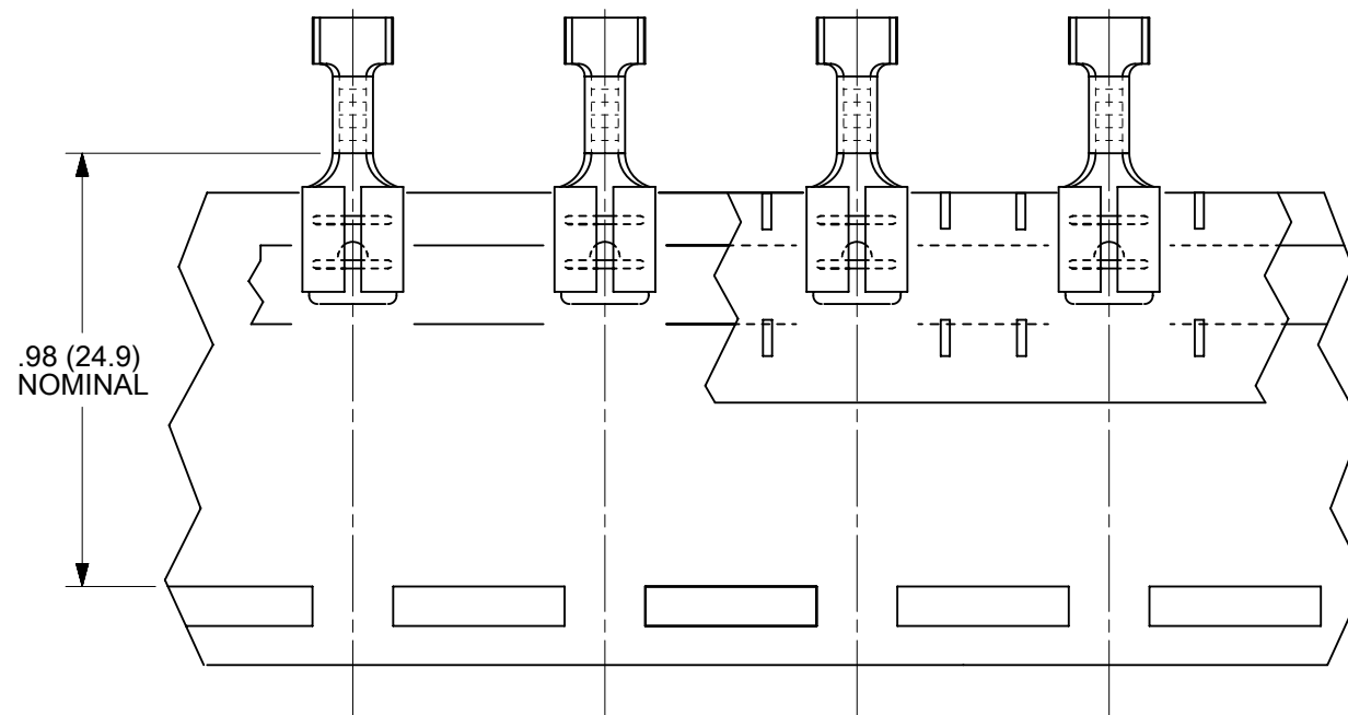
TAPE-MOUNTED PARTS
