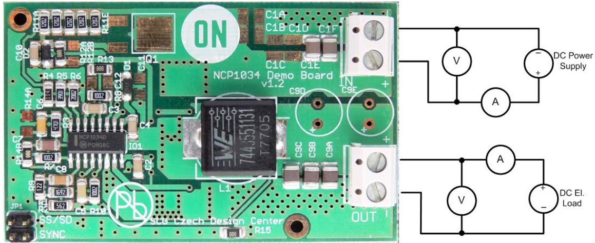
Figure 1: Test Setup
