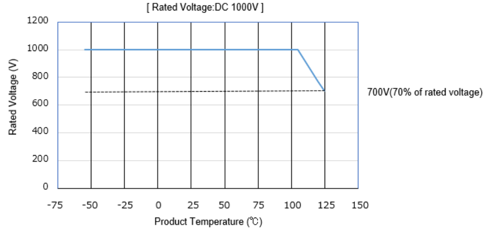
Fig:Derating
