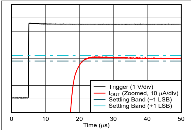
Figure 6-43. Current Output Settling Time: Rising Edge (1/4 to 3/4 scale)
