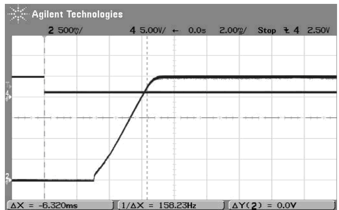
On/Off Enable Startup Delay ( V_{in}=12V, V_{out}=2.5V, I_{out}=3A, C_{load}=0 ) Trace 4=Enable In, Trace 2=Vout
