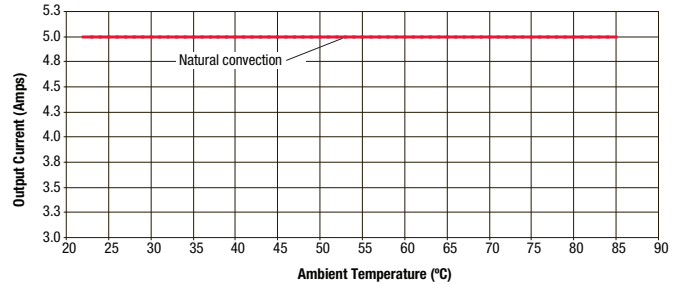
OKY-T/5-D12 Maximum Current Temperature Derating @ Sea Level ( V_{in} = 12V, V_{out} = 1.5V , airflow is transverse)
