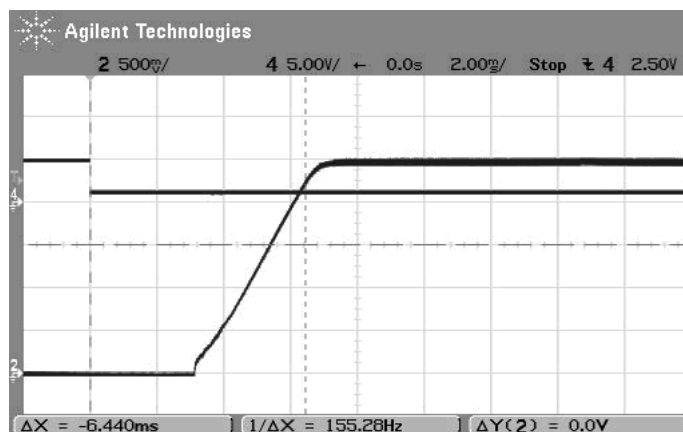
On/Off Enable Startup Delay (Vin=12V, Vout=2.5V, Iout=5A, Load=0) Trace 4=Enable In, Trace 2=Vout
