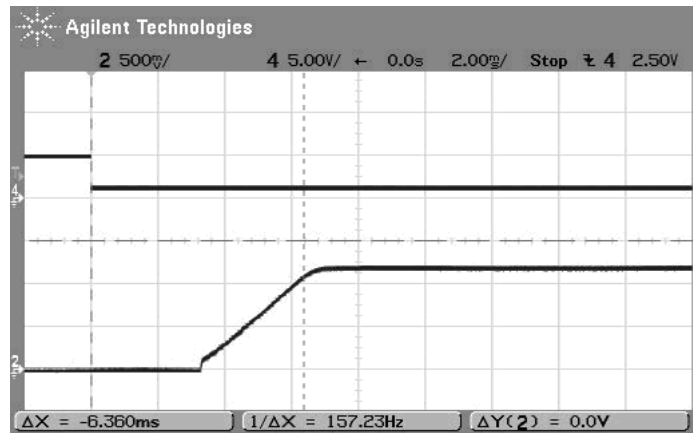
On/Off Enable Startup Delay ( V_{in}=12V, V_{out}=1.2V, I_{out}=3A, C_{load}=0 ) Trace 4=Enable In, Trace 2=Vout
