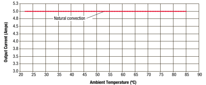
OKY-T/5-D12 Maximum Current Temperature Derating @ Sea Level (Vin = 12V, Vout = 5V, airflow is transverse)
