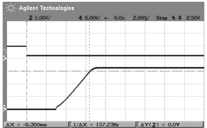
On/Off Enable Startup Delay (Vin=12V, Vout=3.3V, Iout=0.04A, Cload=0) Trace 4=Enable In, Trace2=Vout
