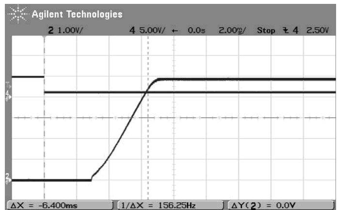
On/Off Enable Startup Delay (Vin=12V, Vout=5V, Iout=5A, Cload=0 Trace 4=Enable In, Trace2=Vout)
