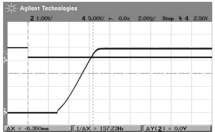
On/Off Enable Startup Delay (VIN=12V, Vout=5V, Iout=3A, Cload=0) Trace 4=Enable In, Trace2=Vout
