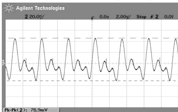
Output Ripple and Noise (Vin=12V, Vout=2.5V, Iout=5A, Load=0, ScopeBW=100MHz)
