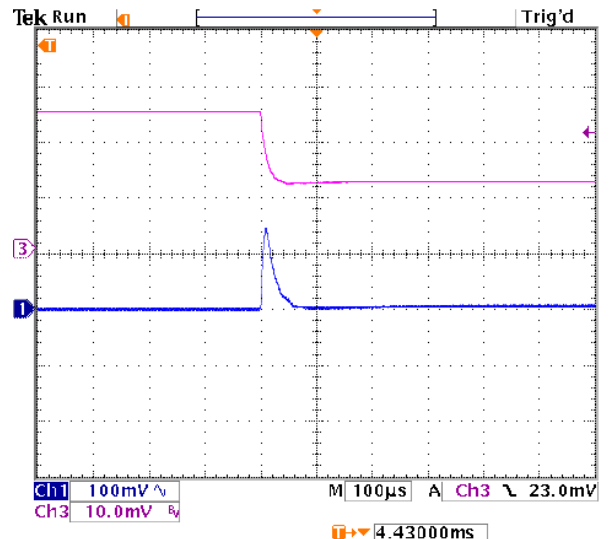
Step Load Transient Response (Vin=12V, Vout=5V, Cload=0, Iout=5A to 2.5A) Trace 1=Vout, 100 mV/div. Trace 3=Iout, 2A/div.
