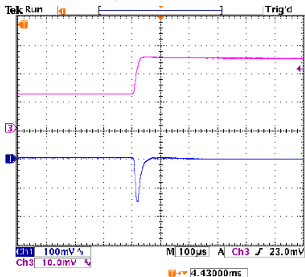
Step Load Transient Response (Vin=12V, Vout=2.5V, Load=0, Iout=2.5A to 5A) Trace 1=Vout, 100 mV/div. Trace 3=Iout, 2A/div.
