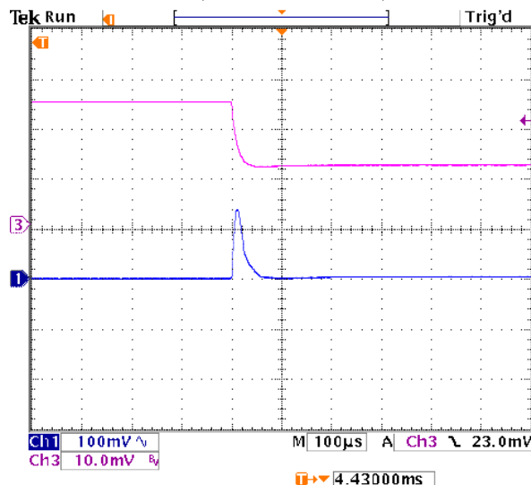
Step Load Transient Response (Vin=12V, Vout=2.5V, Load=0, Iout=5A to 2.5A) Trace 1=Vout, 100 mV/div. Trace 3=Iout, 2A/div.
