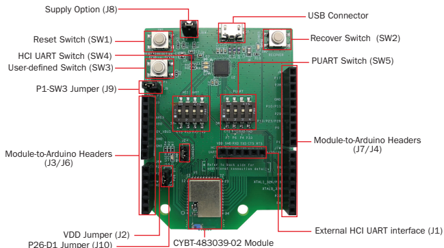
Figure 1: CYBT-483039-EVAL Top View
