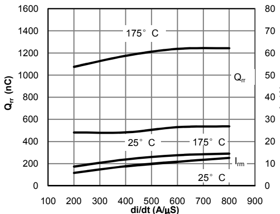
Fig 25: Diode Reverse Recovery Charge and Peak Current vs. di/dt ( V_{GE}=15V, V_{CE}=400V, I_F=15A )
