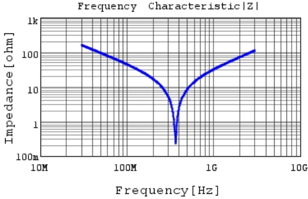
RCE7U3A330J2K1H03B |Z| DC0V, 25degC
