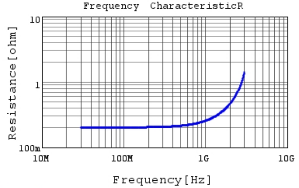
RCE7U3A330J2K1H03B R DC0V, 25degC
