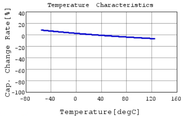
RCE7U3A330J2K1H03B C-Temp. capchange, DC0V,
