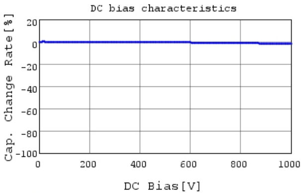
RCE7U3A330J2K1H03B C-DC bias capchange, 25.0
