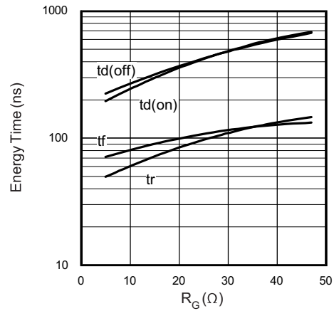
Fig. 10 - Typical Switching Time vs. R_g , T_J = 125\text{ }^\circ\text{C} , L = 200\text{ }\mu\text{H} , V_{CC} = 360\text{ V} , I_{CE} = 100\text{ A} , V_{GE} = 15\text{ V}
