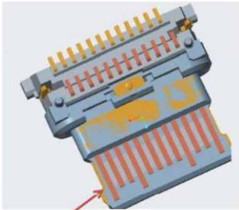
Old Grounding plate thickness 0.20mm
