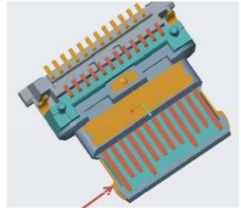
New Grounding plate thickness 0.15mm
