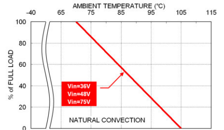
RCD15-48 Derating Curve
