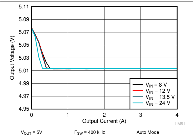
Figure 9-12. LM61440 Load and Line Regulation
