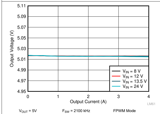
Figure 9-15. LM61440 Load and Line Regulation
