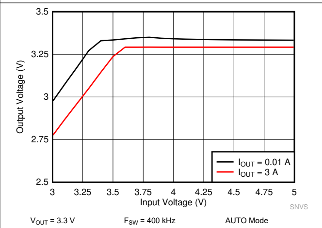
Figure 9-16. LM61440 Dropout Curve
