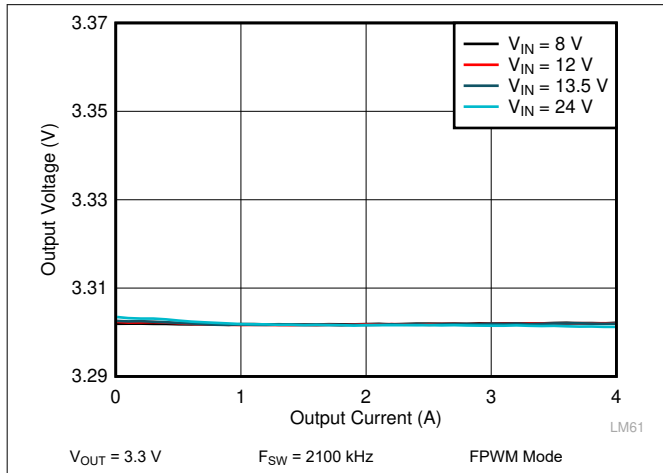
Figure 9-11. LM61440 Load and Line Regulation
