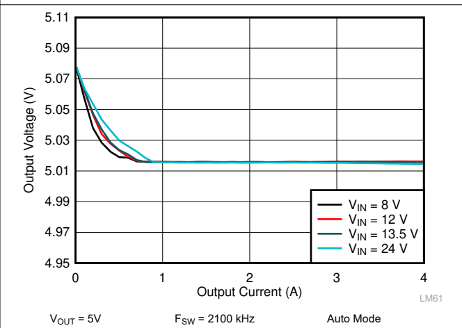
Figure 9-14. LM61440 Load and Line Regulation
