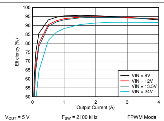
Figure 9-7. LM61440-Q1 Efficiency
