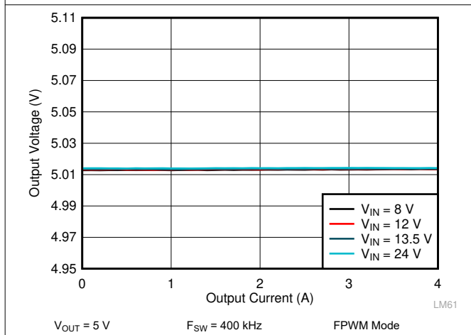
Figure 9-13. LM61440 Load and Line Regulation
