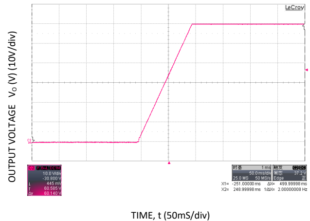
Figure 10. 65V DC soft start, full load, V IN = 230V AC - I 2 C mode with 4700μf external capacitance.
