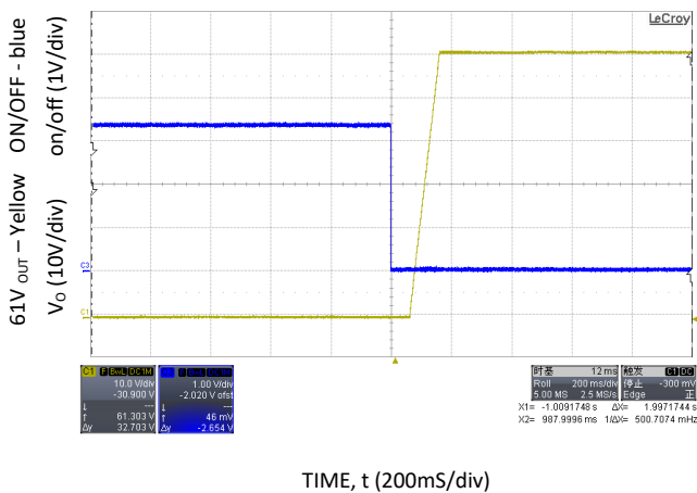
Figure 9. 65V DC soft start delay when ON/OFF is asserted, V IN =230V AC - I 2 C mode.
