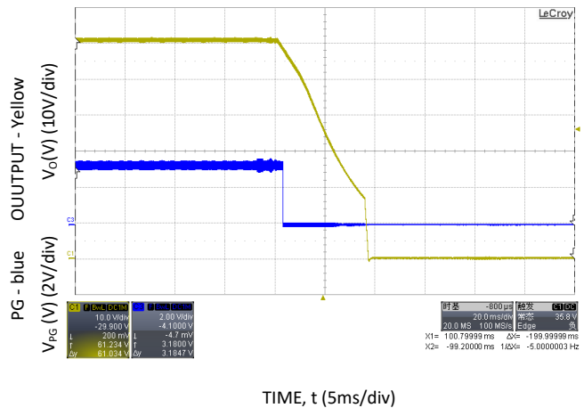
Figure 12. PG# alarmed 10ms prior to V o < 30V, V IN = 230V AC , Output at Full load
