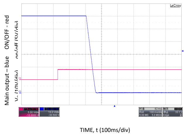
Figure 16. 65V DC turn-OFF delay when ON/OFF is di-asserted, V_{IN}=230V_{AC} - I 2 C mode.
