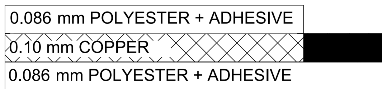
0.155 mm POLYESTER CROSS-SECTION
