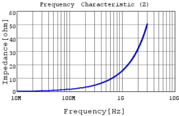
LQG15WH2N5C02 |Z|
