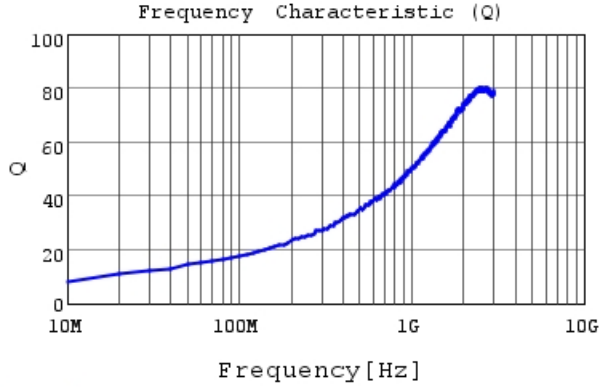
LQG15WH2N5C02 Q
