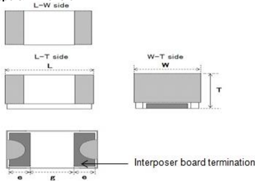
image:Dimension
