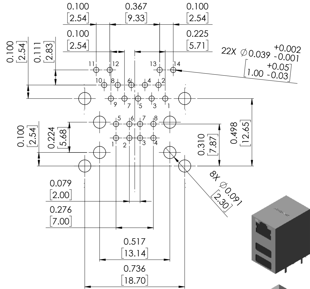
Recommended Hole Pattern View From Component Side
