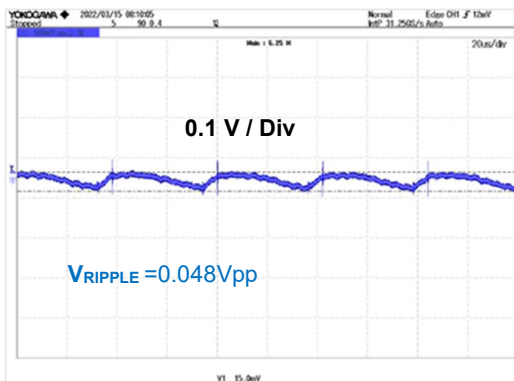
Figure 16. V_{IN} = 90 \text{ Vac} , I_{OUT} = 0.4 \text{ A}
