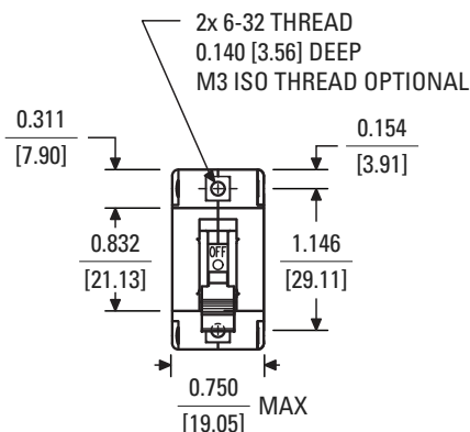
Single Pole
