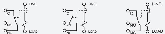
Series with Auxiliary Switch
