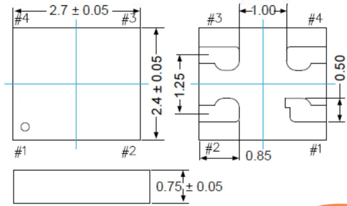
2.7 x 2.4mm Package (Option "D", compatible with 2.5 x 2.0mm footprint)
