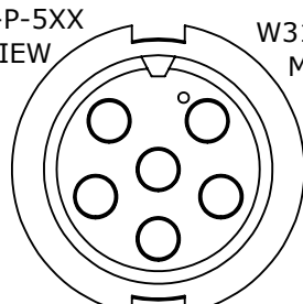
W3382-6SG-P-5XX MATING VIEW
