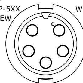
W3382-5SG-P-5XX MATING VIEW
