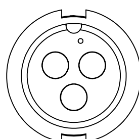
W3182-3SG-P-5XX MATING VIEW
