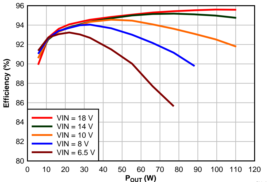
BOOST CV 2-Phase Efficiency vs P_{OUT} (W)
