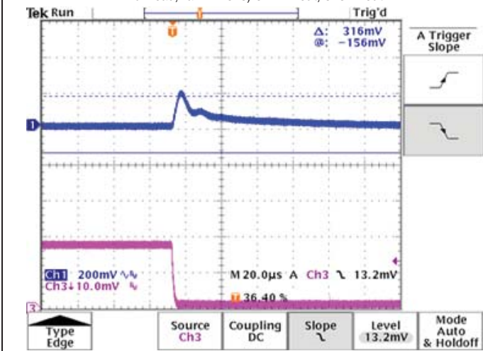
Step Load Transient Response (Vin = 12V, Vout = 3.3V, Cloud = 1000µf, Iout = 0% to 50% of full load, Ta = +25°C) Ch1 = Vout, Ch3 = Iout
