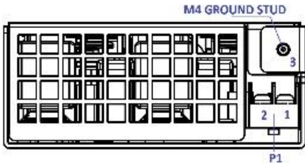
Figure 5. Front View - MBC1200-1T24-PCF Model
