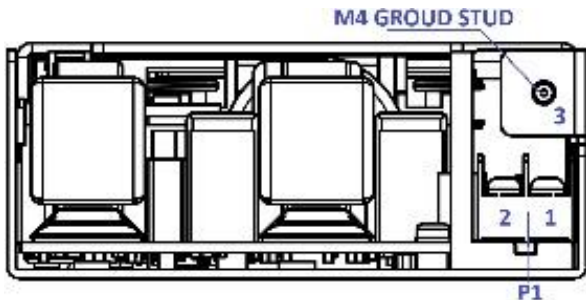
Figure 2. Front View - MBC1200-1T24-UCF Model
