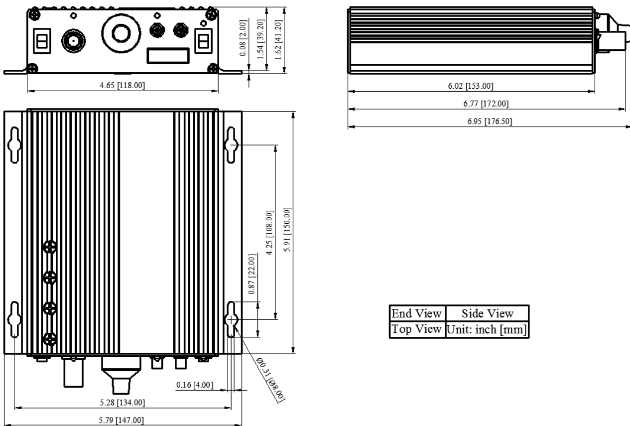
Figure 12. Dimensions of AHVA2KV2X5MA
