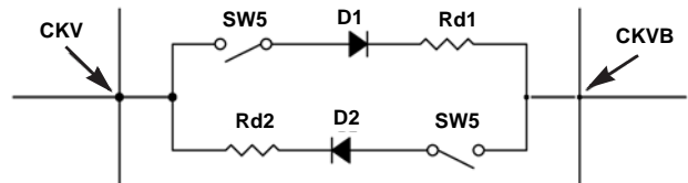
FIGURE 18. BI-DIRECTIONAL SWITCHES
