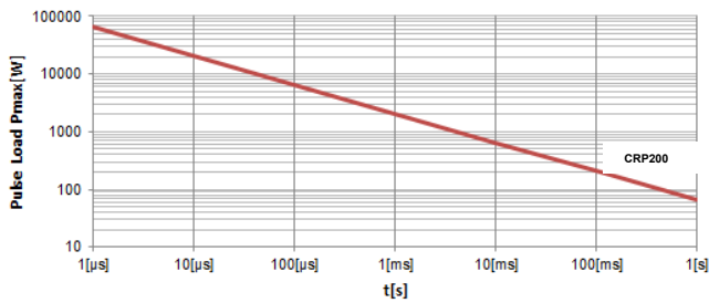
POWER CURVE
