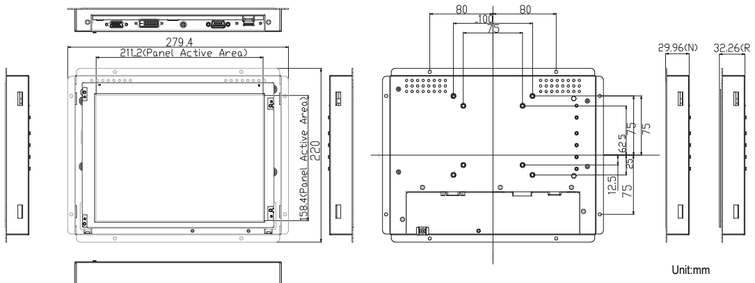
Figure 2.1 IDS-3110 Series Dimensions
