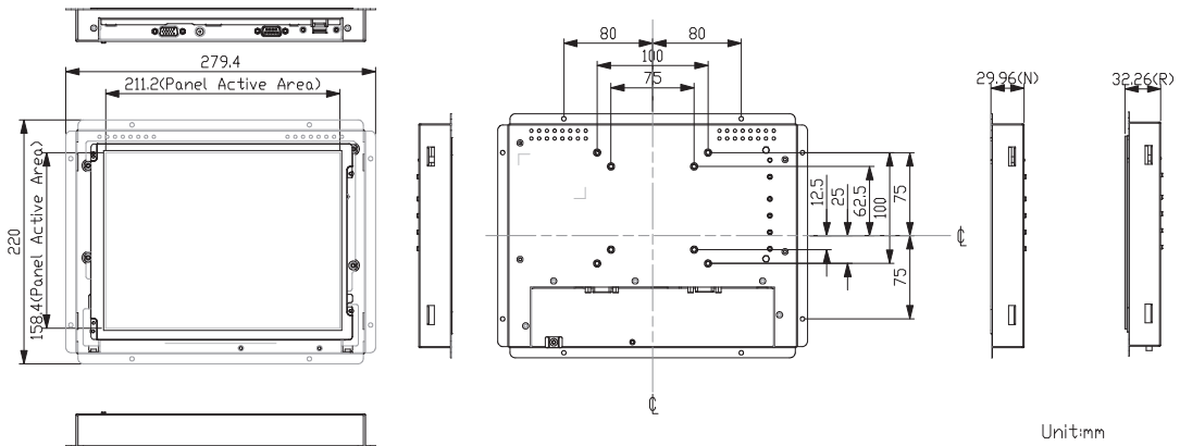
Figure 2.2 IDS-3110E Series Dimensions
