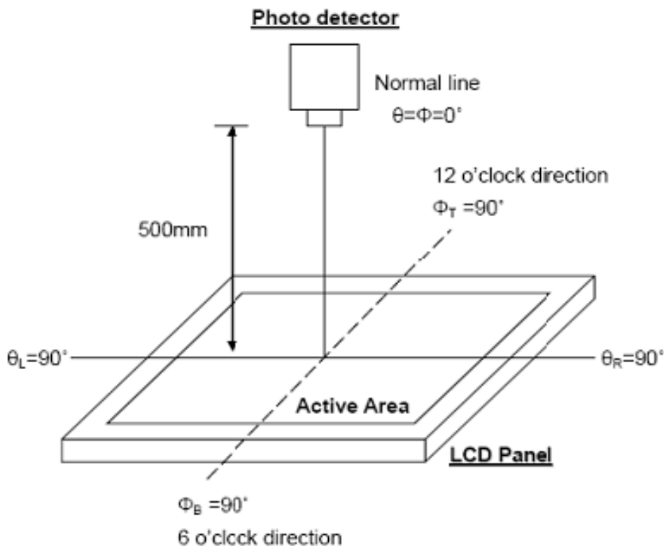
Fig. 9-2 Optical measurement system setup
