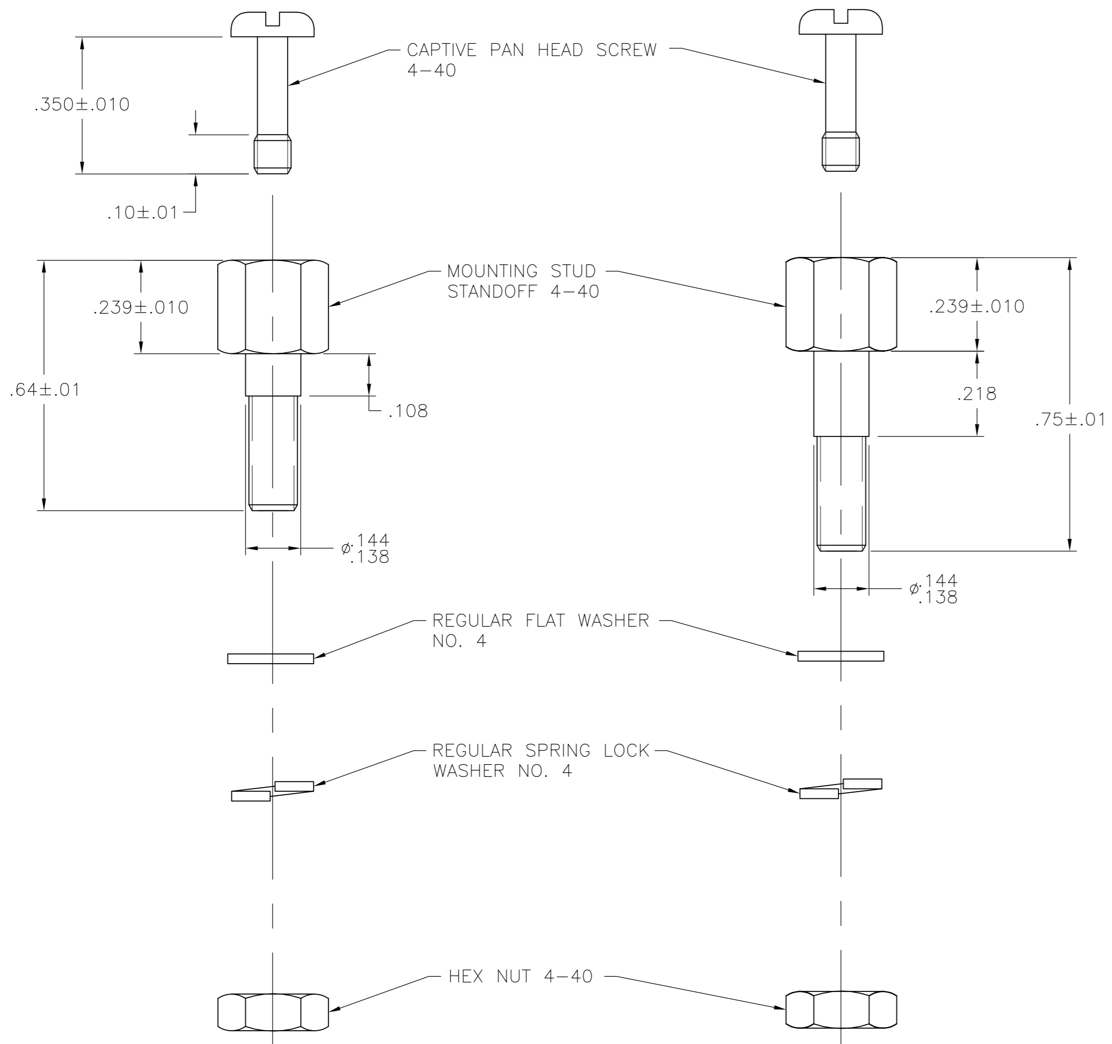
KIT P/N 5552568-2 VIEW B
