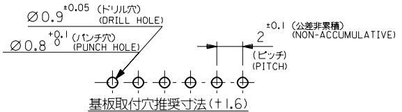
基板取付穴推奨寸法(+1.6) RECOMMENDED PC BOARD HOLE DIMENSION(+1.6)
