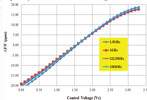
Frequency Pull Vs. Control Voltage (LVDS Output)
