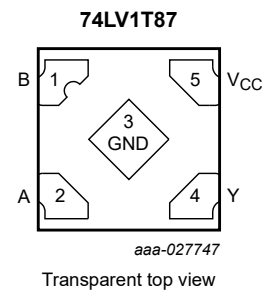
Fig. 5. Pin configuration SOT1226-3 (X2SON5)
