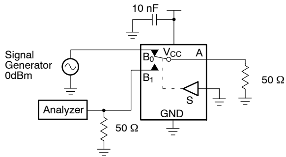
Figure 17. Crosstalk
