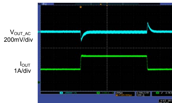
Time 200µs/div
