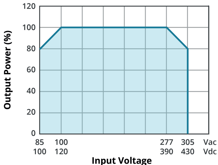
INPUT VOLTAGE DERATING CURVE (25°C)
