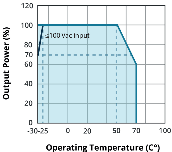
TEMPERATURE DERATING CURVE
