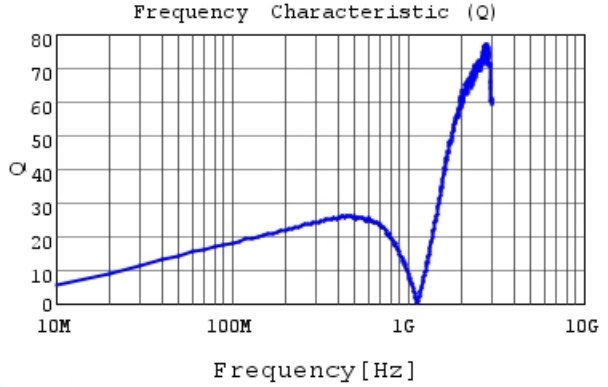
LQG15WHR13J02 Q
